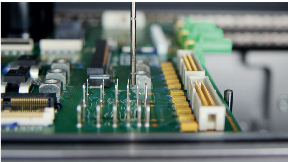
Precise coating of electronic connections between tightly packed, tall components
